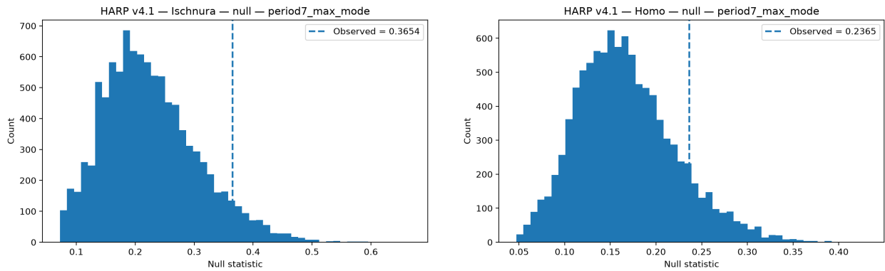
Figure 4: Permutation test for seven-residue periodic organisation of MyhT–IBAM contact occupancy in Ischnura and Homo . Histograms show the null distributions obtained after repeatedly disrupting the correspondence between MyhT sequence position and the DeepCoil2-anchored heptad register while preserving the underlying contact information. The dashed vertical line marks the period7_max_mode statistic measured from the unpermuted trajectory-derived data. This statistic asks whether the distribution of MyhT–IBAM contacts contains a stronger seven-residue periodic component than would normally arise after the register relationship has been randomized. In Ischnura (left), the observed statistic (0.3654) lies well into the upper tail of the null distribution, indicating pronounced seven-residue periodic organisation. Homo (right) likewise shows an observed statistic (0.2365) displaced toward the upper tail, although the separation from its null distribution is less extreme. Thus, both taxa contain evidence that contact occupancy is structured according to the expected heptad periodicity rather than being distributed arbitrarily along the MyhT sequence. The figure tests periodicity, not whether a particular heptad phase is preferentially occupied; the latter is addressed separately by the phase-specific analyses.
