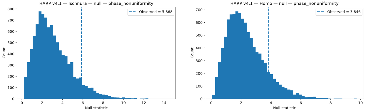
Figure 5: Permutation test for non-uniform distribution of MyhT–IBAM contacts among DeepCoil2-anchored heptad phases in Ischnura and Homo . Histograms show the null distributions obtained after repeatedly disrupting the relationship between the trajectory-derived MyhT contact pattern and its DeepCoil2-defined heptad register. The dashed vertical line indicates the phase_nonuniformity statistic calculated from the observed, unpermuted data. This statistic measures how strongly contact occupancy is concentrated in particular heptad phases rather than being distributed approximately evenly among phases a–g. Ischnura (left) has an observed non-uniformity statistic of 5.868, lying well toward the upper tail of its null distribution. This reflects the strongly unequal phase occupancy seen in Figures 02–03, particularly the enrichment of phase c and depletion of phase d. Homo (right) also exhibits greater phase non-uniformity than is typical under the null model, with an observed statistic of 3.846, although its displacement is less pronounced than that of Ischnura . These results demonstrate that the phase-specific contact distributions are more uneven than would ordinarily be expected after the correspondence between contact position and heptad register has been disrupted. This test evaluates how unevenly contacts are distributed among the seven phases; it does not by itself specify which phase is preferred or test seven-residue periodicity.
