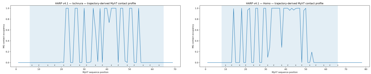
Figure 1: Trajectory-derived MyhT contact profiles for Ischnura and Homo. MyhT-IBAM major-groove (MG) contact occupancy is plotted as a function of MyhT sequence position for representative Ischnura (left) and Homo (right) trajectories. The shaded region denotes the DeepCoil2-defined coiled-coil interval, with the predicted a and d heptad positions shown along the sequence axis. Contact occupancy ranges from 0 (no MG contact during the sampled trajectory) to 1 (persistent contact), thereby converting the molecular-dynamics trajectory into a residue-resolved description of where MyhT engages the IBAM major groove. Both taxa show highly non-uniform contact profiles, with contacts concentrated within particular portions of the DeepCoil2-defined interval rather than distributed uniformly along MyhT. Importantly, the detailed profiles differ between Ischnura and Homo, illustrating that HARP begins with taxon-specific trajectory-derived contact behaviour rather than imposing a common interaction pattern. These residue-level profiles provide the empirical input that is subsequently projected onto the DeepCoil2-anchored a-g heptad coordinate system for phase-level analysis.
