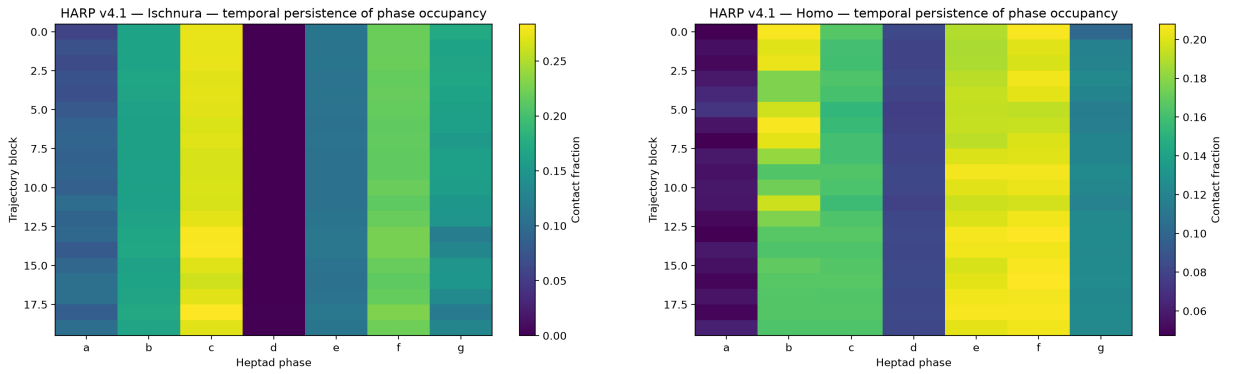
Figure 3: Temporal persistence of DeepCoil2-anchored heptad-phase contact occupancy in Ischnura and Homo . The molecular-dynamics trajectory is divided into sequential time blocks (rows), and MyhT-IBAM major-groove contact occupancy is recalculated for each DeepCoil2-defined heptad phase (a–g, columns). Colour represents the fraction of contact assigned to each phase within that trajectory block, allowing the phase preferences summarised in Figure 02 to be examined through time rather than only as trajectory-wide averages. Ischnura (left) exhibits a remarkably persistent pattern dominated by phase c, with substantial f occupancy and essentially absent d occupancy throughout the trajectory. Homo (right) displays a broader distribution, principally involving b, c, e, and f, while a and d remain comparatively depleted. Although local fluctuations occur between trajectory blocks, the major phase preferences remain recognizable throughout the simulation. The heatmaps therefore demonstrate that the non-uniform phase distributions in Figure 02 are temporally persistent features of the trajectory rather than averages produced by a small number of transient contact events. Importantly, the different colour scales should be read independently: colour intensity is used to reveal temporal structure within each taxon and should not be used for direct quantitative comparison between taxa.
