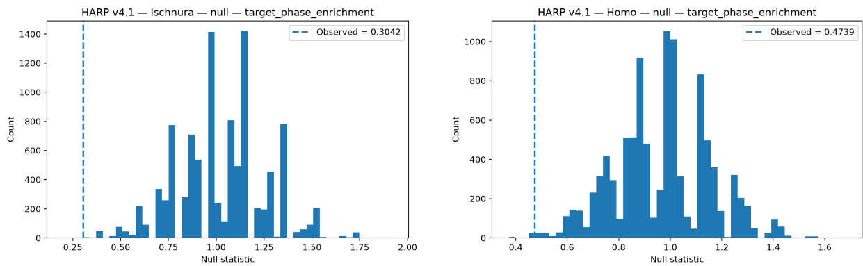
Figure 6: Permutation test for enrichment of MyhT–IBAM contacts at the predefined target heptad phases in Ischnura and Homo . Histograms show the null distributions generated by repeatedly disrupting the correspondence between the trajectory-derived MyhT contact pattern and its DeepCoil2-anchored heptad register. The dashed vertical line represents the target_phase_enrichment statistic calculated from the observed, unpermuted data. Unlike the preceding tests, which ask whether contacts exhibit seven-residue periodicity (Figure 04) or are distributed non-uniformly among heptad phases (Figure 05), this test asks whether contacts are specifically enriched at the predefined target phase relationship. In both Ischnura (left; observed = 0.3042) and Homo (right; observed = 0.4739), the observed statistic lies toward the lower extreme of the corresponding null distribution. Thus, although both taxa exhibit structured and non-uniform heptad-associated contact patterns, that organisation does not take the form of enrichment at the particular target phases represented by this statistic. Figure 06 therefore distinguishes general heptad organisation from conformity to a specific hypothesised phase arrangement.
